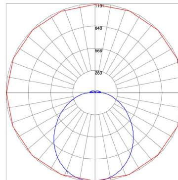
TSS 4 30/40/50 G1 FSK Lumen setting (30 - 3120 LM) CCT setting 3500K Wattage (24W)
